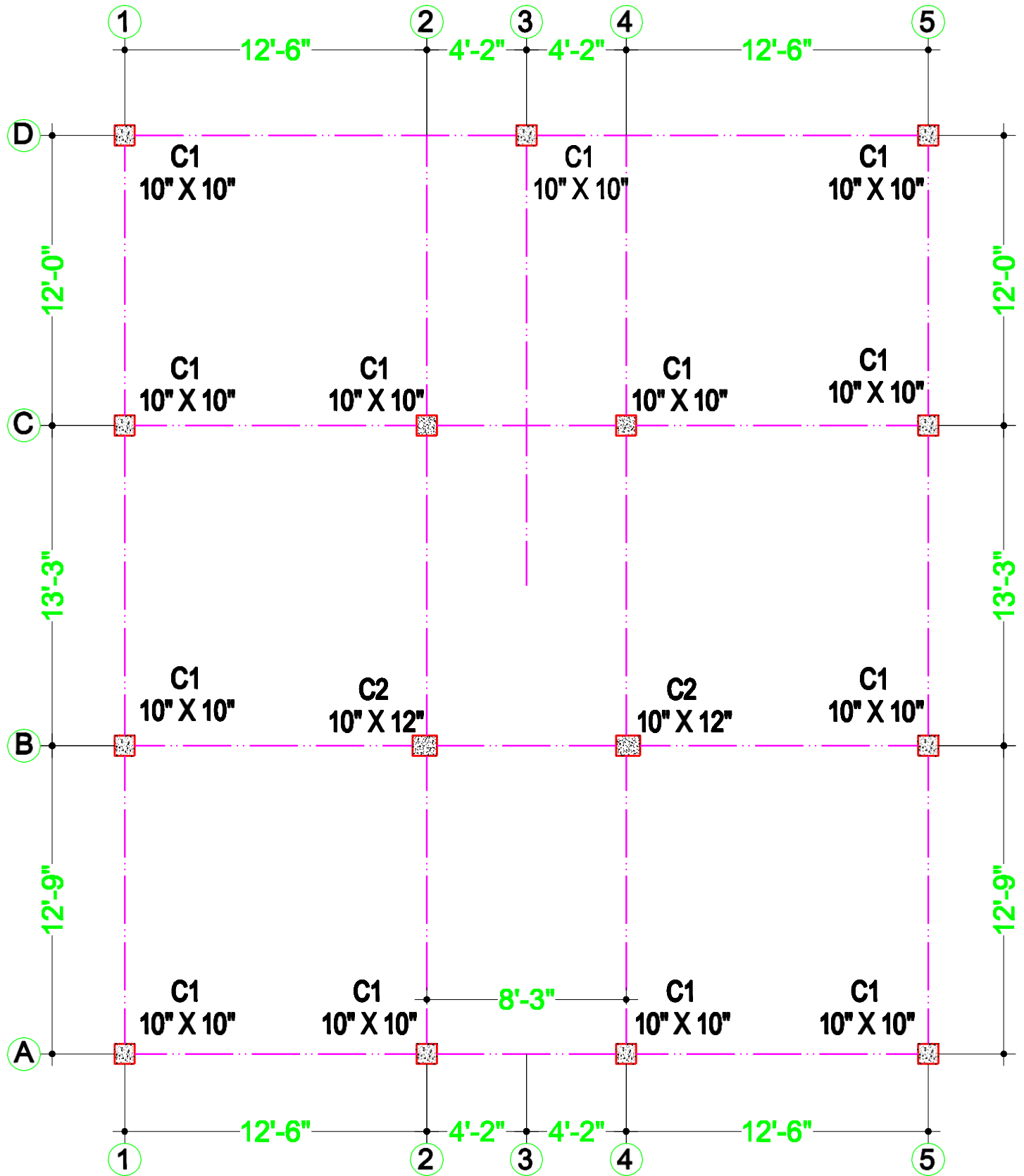
COLUMN LAYOUT
