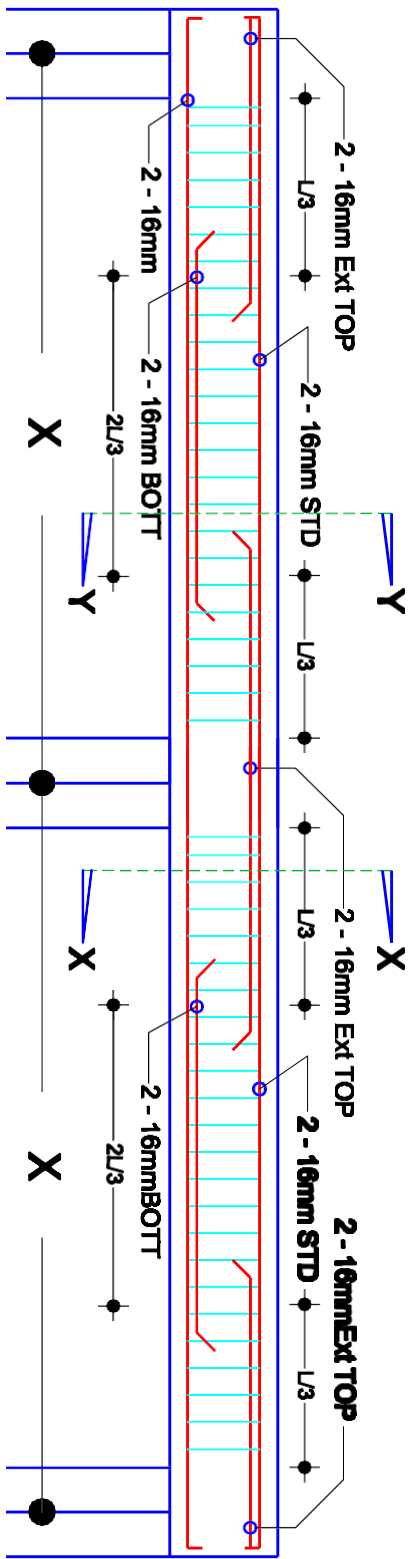
Long Sec. of F.B - 01 ( 10" X 12" )
