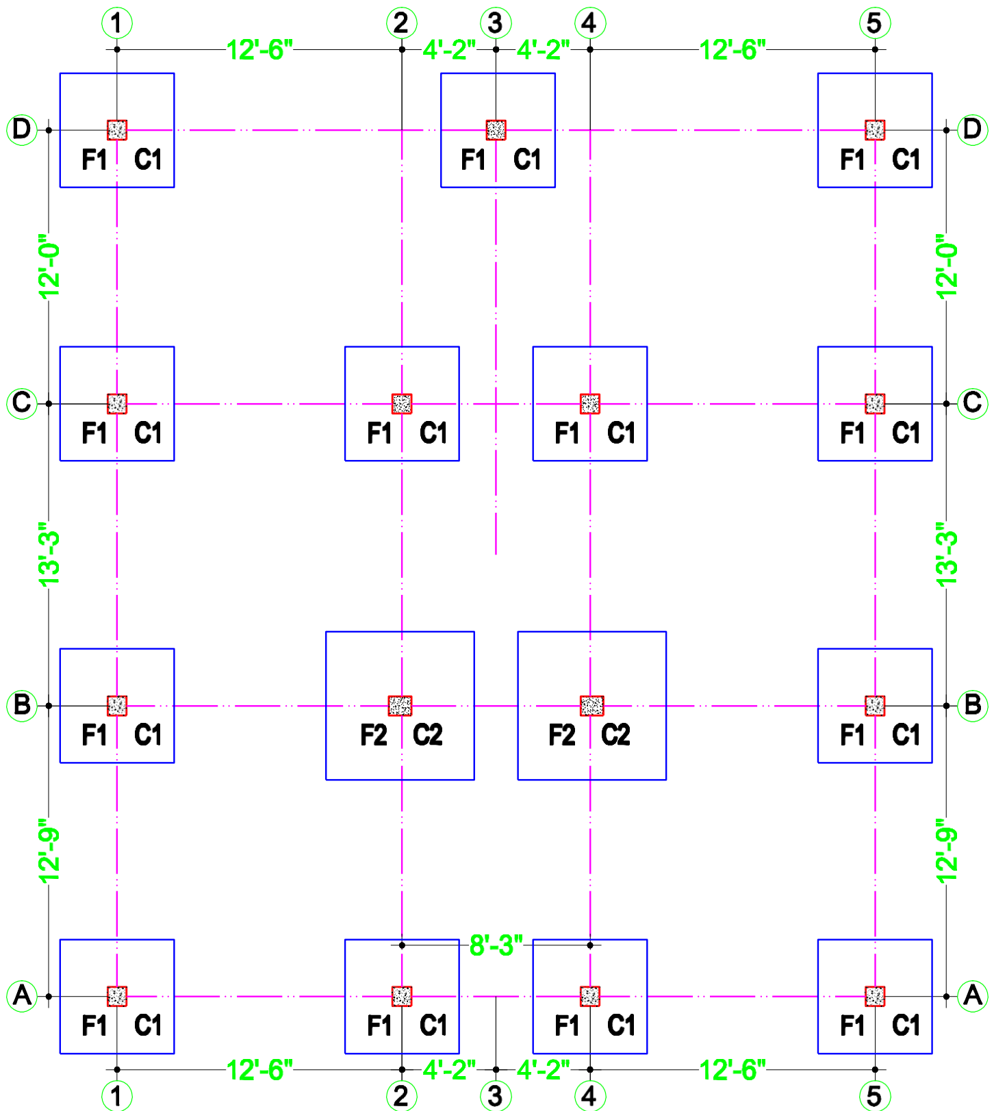
FOOTING LAYOUT
